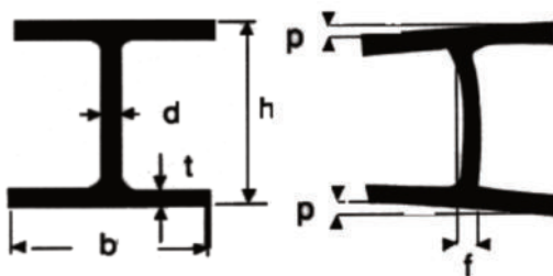
HEA (DIN 1025/3) HEB (DIN 1025/2)
